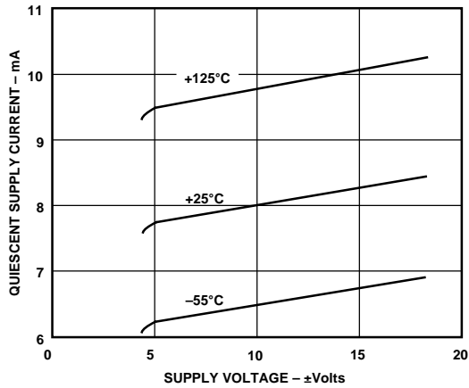
Figure 7. Quiescent Supply Current vs. Supply Voltage
