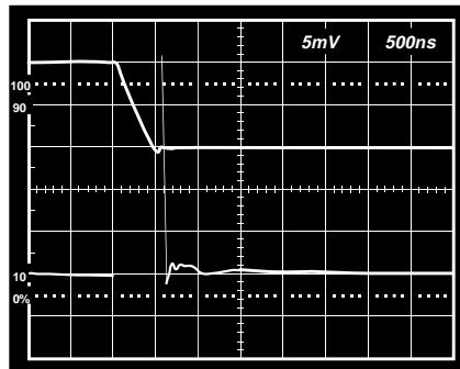
Figure 25. 16-Bit Settling Time Positive Input Pulse
