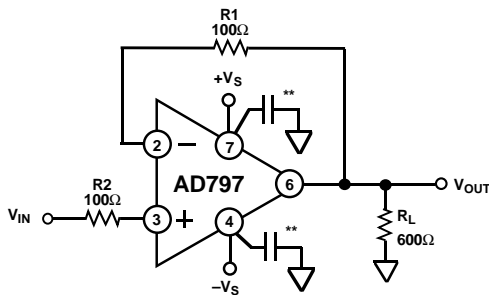
Figure 33. Voltage Follower Connection
