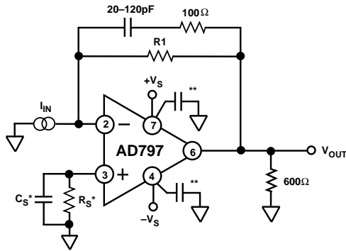
Figure 36. I-to-V Converter Connection
