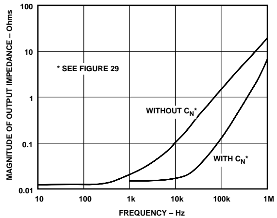
Figure 18. Magnitude of Output Impedance vs. Frequency
