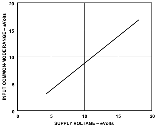
Figure 1. Common-Mode Voltage Range vs. Supply
