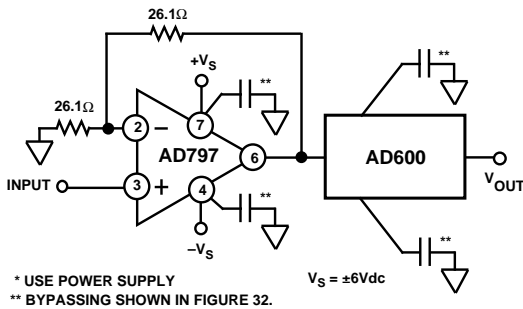
Figure 47. An Ultrasound Preamp Circuit
