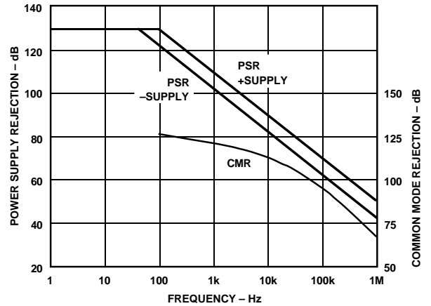
Figure 10. Power Supply and Common-Mode Rejection vs. Frequency
