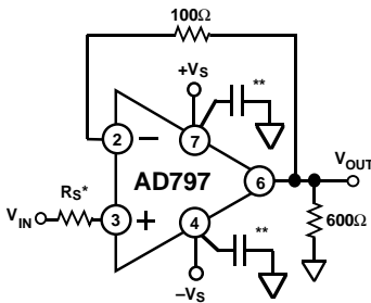
Figure 22. Follower Connection
