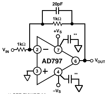
Figure 19. Inverter Connection
